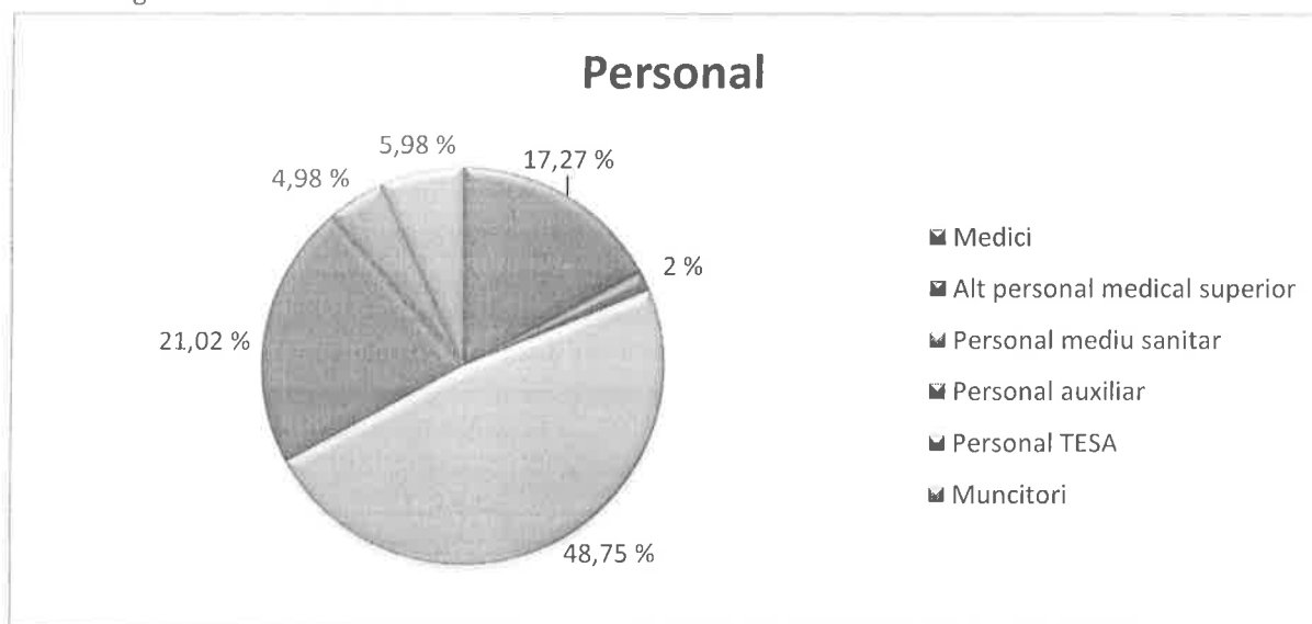
Fig. 1 – Grafic Personal
